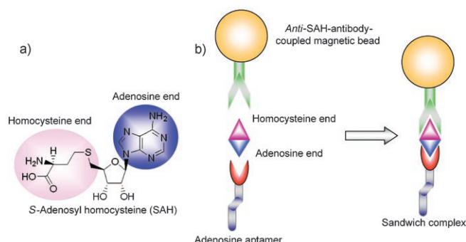
Figure 1. Sandwich complex formation: a) Structure of S-adenosyl homocysteine (SAH); b) Binding of anti-SA-antibody-coupled magnetic bead to the homocysteine end of SAH produces a sandwich complex after binding of the adenosine-specific aptamer to the adenosine end of SAH.
